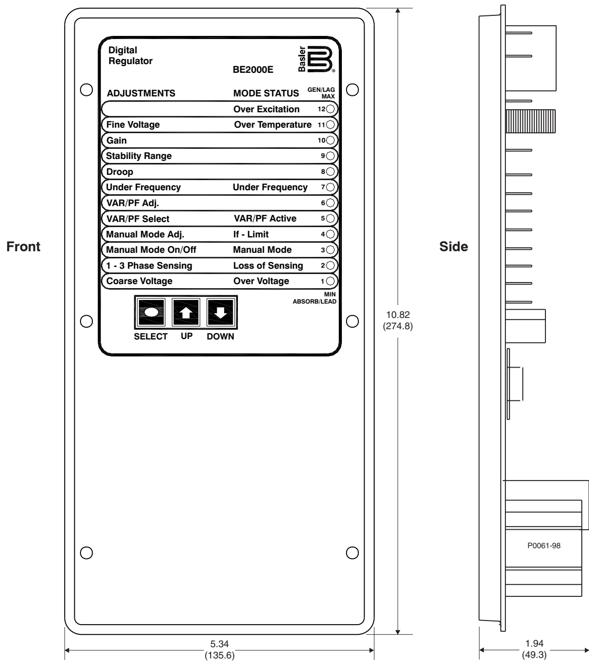
Figure 2 - Dimensions
